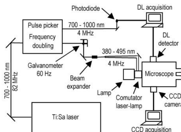
FIGURE 1 Delay line set-up for picosecond fluorescence decay microscopy. A picosecond Ti:Sapphire laser after pulse picker and frequency doubling delivered 4 MHz repetitive rate pulses at a tunable 380–495 nm wavelength. The fundamental laser rejected from frequency doubling (4 MHz repetitive rate) was used to trigger an ultrafast photodiode (Hamamatsu, Photonics France, Massy, France). The excitation laser beam was transformed by a galvanometer-beam expander system before entering the microscope. A rotating mirror was used as a commutator between lamp and laser excitation. Two outputs of the microscope are used for CCD camera and DL detection. The photodiode signal was used by the DL acquisition to characterize the time difference between the pulse laser and the single photon emission counted by the detector.
